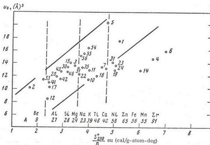
Fig. 3. \bar{S}_{298}^0 (mean standard entropy) in relation to v_0 . The numbers are those of the minerals in Table 1.
