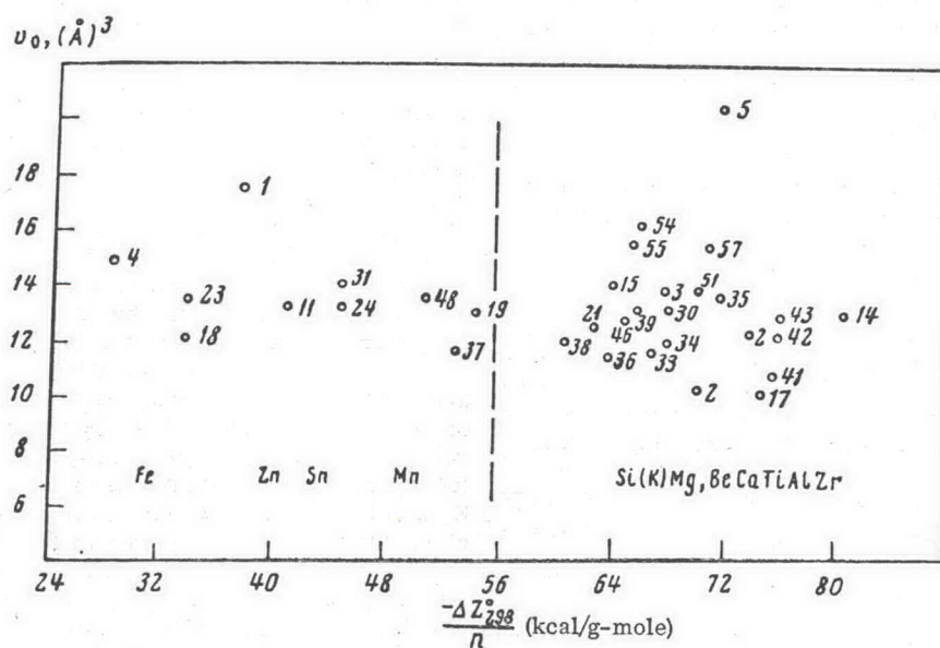
Fig. 4. Mean Gibbs free energy -\Delta Z_{298}^0/n in relation to v_0 . The numbers are those of the minerals in Table 1.
